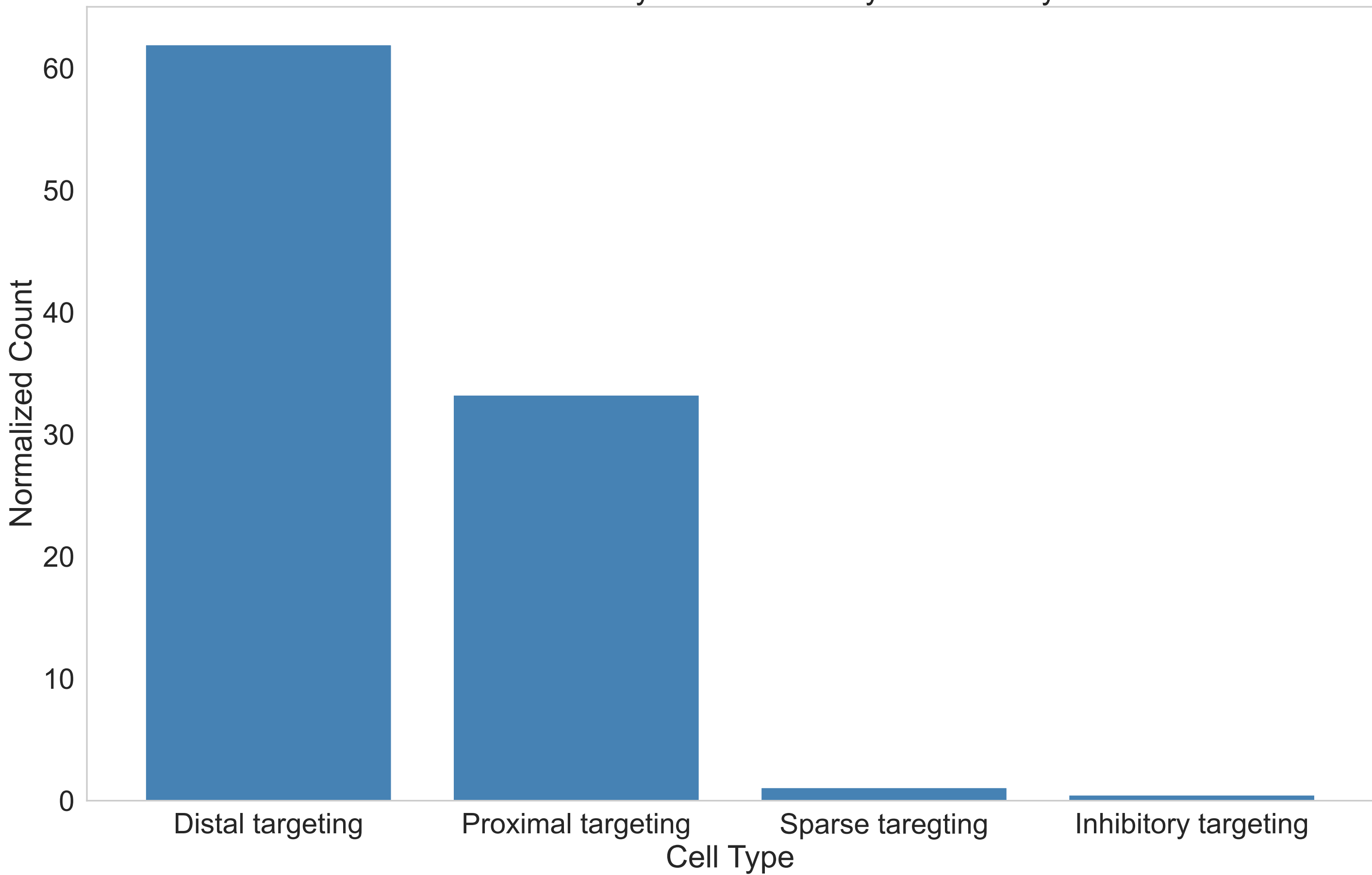
Inbound Inhibitory — No Assembly to Assembly
